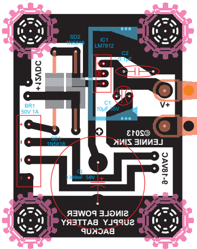
PARTS LAYOUT
