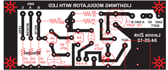
PARTS LAYOUT
