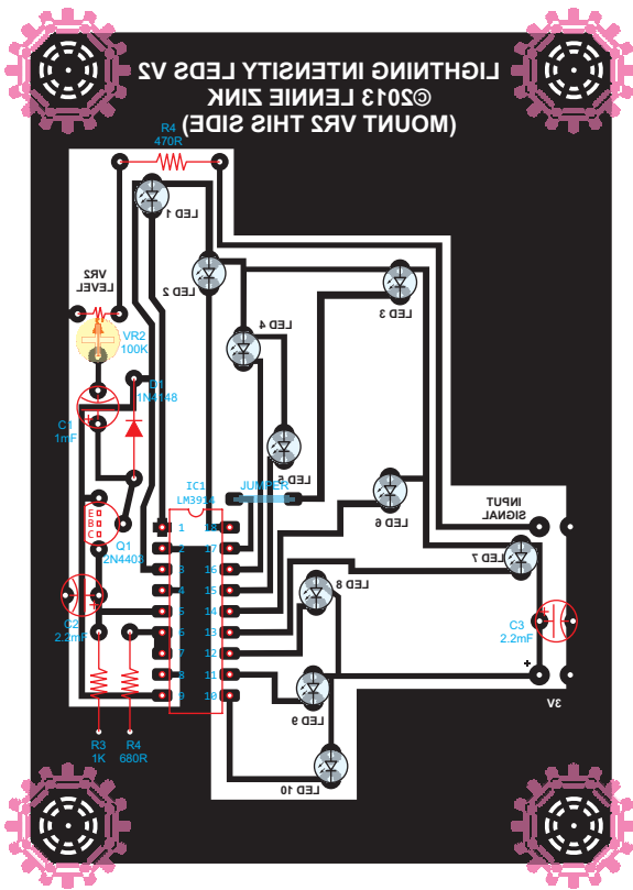
PARTS LAYOUT
