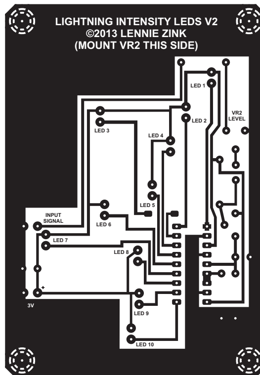
BOTTOM VIEW
