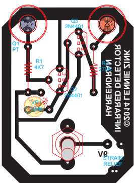
PARTS LAYOUT
