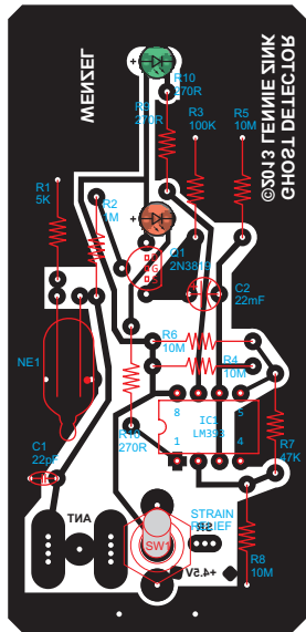
COMPONENT LAYOUT
