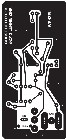
BOTTOM VIEW
