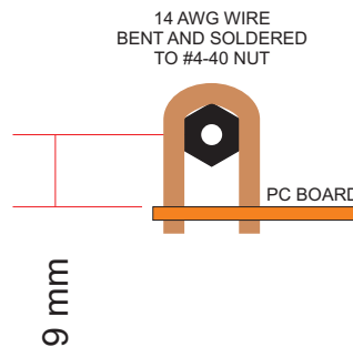
BOTTOM NUT SUPPORT DETAIL
