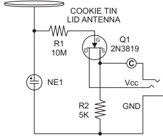
CHARGE SENSOR
