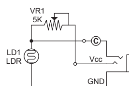
LIGHT SENSOR
