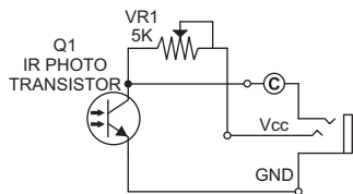
INFRARED SENSOR
